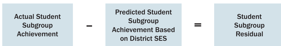
Figure 1 Understanding Residuals
